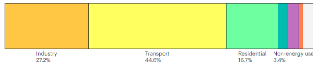
Total final consumption, Mexico, 2023
